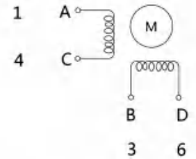
Wiring Diagram
